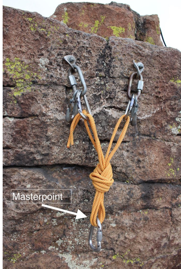
2 point cordelette anchor, bolts
