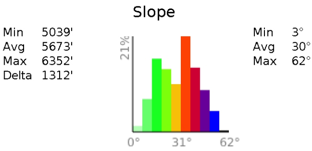
Slope Angle (top), Land Cover (middle), Tree Cover (bottom)
